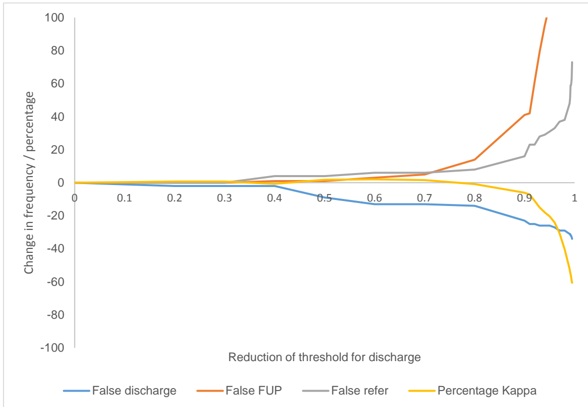
Figure 4.2 Effect of reducing the weight of the naïve Bayes' probability estimate for discharge upon the number of false discharges, false Fups, false refers and percentage Kappa. Reduction of weight was brought about by multiplying the probability estimate by between 1 and 0.005. In order to depict progressively reducing weight from left to right, the value on the horizontal axis is equal to 1 minus the multiplier. The vertical axis has been truncated at 100 to make key elements of the graph clearer (obscuring the full increase in false Fups).
