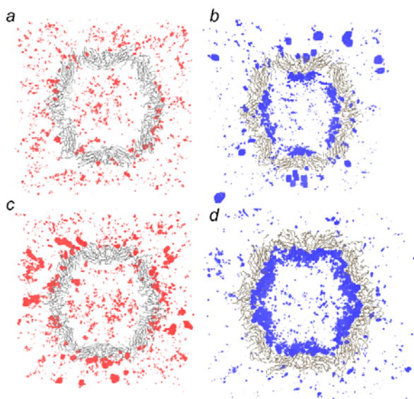
Figure 4. The distribution of ions after the first nanosecond of MD simulation for the low number of ions (top) and for the neutralizing number of ions (bottom). Red density (a,c) represents the density of sodium ions and blue density (b,d) - the density of chloride ions averaged over one nanosecond of simulation. The pictures of the capsids with ions are sliced along the middle of the capsid.
