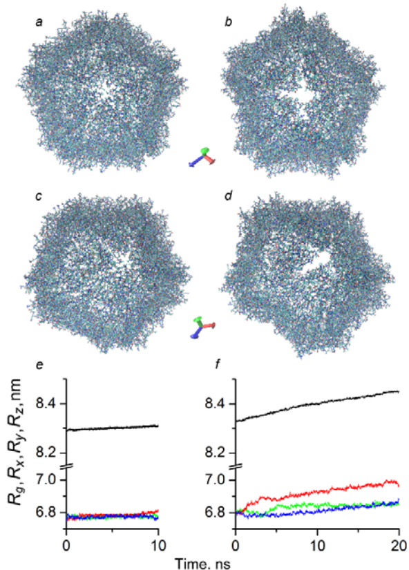
Figure 3. The atomistic structures of PCV2 capsid without tails after simulations: (a,c) the atomistic structures of PCV2 capsid with neutralizing number of ions, (e) radius of gyration for different axis (green is X-axis, red is Y axis, blue is Z axis); (b,d)- the capsid structures with smaller number of ions and (f) radius of gyration for different axis
