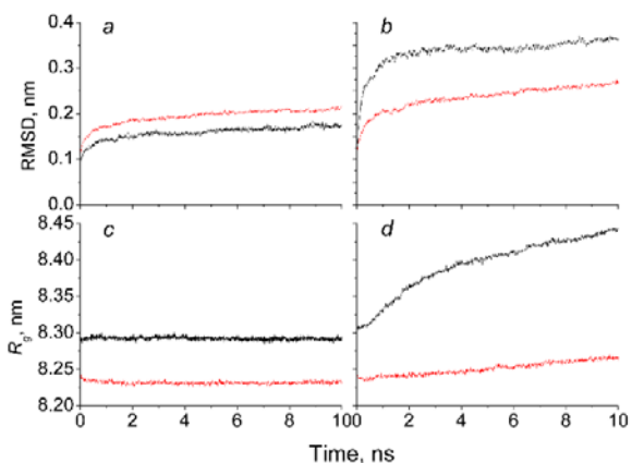
Figure 2. Time change of the root mean square deviation, RMSD , (top plots) and radius of gyration, R_g , (bottom plots) of backbone atoms from their initial structure as a reference structure in AMBER forcefield. The calculations of RMSD and R_g did not include the tail sequence for all structures and consisted of the same number of amino acids. Red is for the capsid with the tails, black is for the capsid without the tails. a,c – the capsids with neutralizing number of ions, b,d – the capsid with low number of ions
