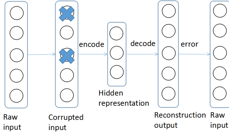
Fig. 3. A graphic structure of SDAE.
