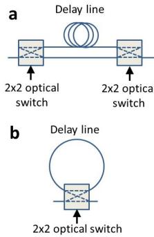
Figure 1. Illustration of a feedforward optical buffer (a) and a feedback optical buffer (b).
