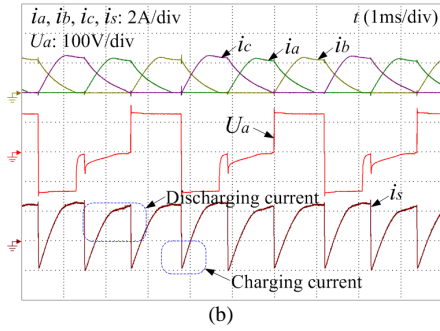
Fig. 19. Experimental results for high-speed operation. (a) Powered by the generator. (b) Powered by the dual-source.
