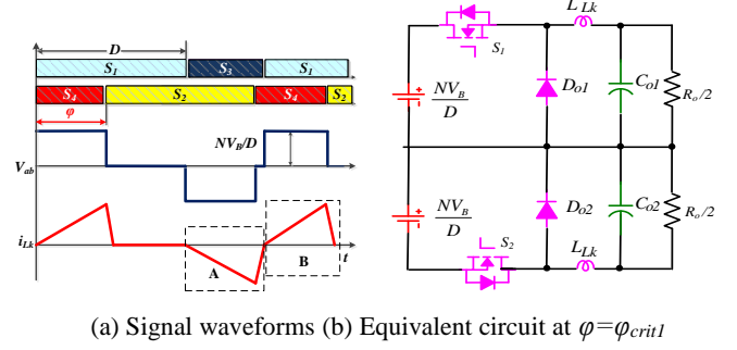
Fig. 7. System operation in Case 1.
