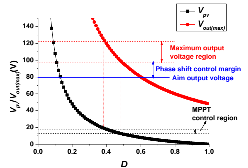
Fig. 10. Design considerations.
