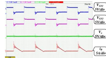
Fig. 16. Steady-state waveforms under mode 3.
