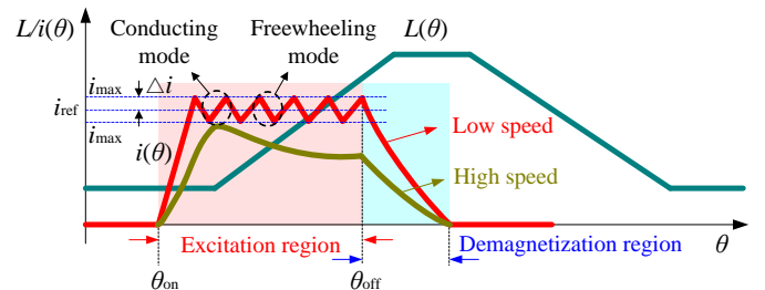
Fig. 4. Phase currents at low and high speeds.
