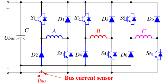
Fig. 7. BCS placement strategy.
