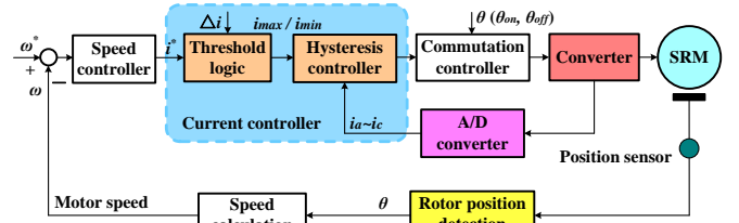
Fig. 3. Control diagram for closed-loop SRM drives with current hysteresis control.
