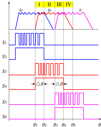
Fig. 5. Phase currents and gate signals under CCC in low-speed operation.
