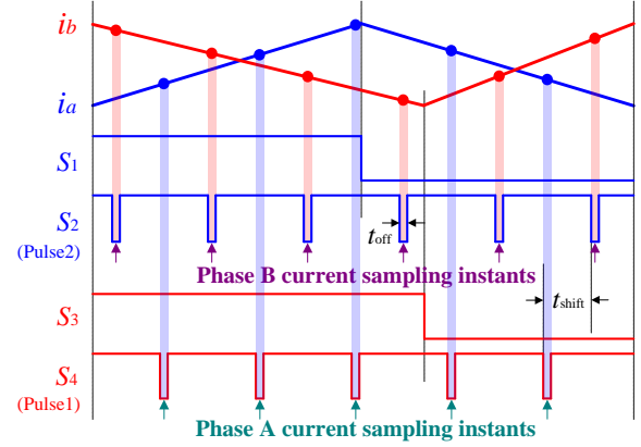
Fig. 9. Diagram of pulse1 and pulse2 injections into the lower-transistors of phases A and B in the current overlapping region for excitation current sampling and decoupling.
