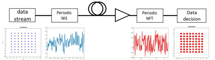
Fig. 2: Blueprint of the PNFT-based communication system. Data stream is mapped on the NS (here it is the main spectrum) and the signal in the time domain at the transmitter is constructed from this main spectrum via the inverse PNFT. At the receiver side, by performing the direct PNFT one retrieves the initial data.
