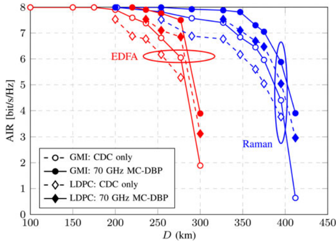
Fig. 6. AIR versus distance ( D ) using EDFA and Raman system. CDC only and 70 GHz MC-DBP BW performance is also displayed.
