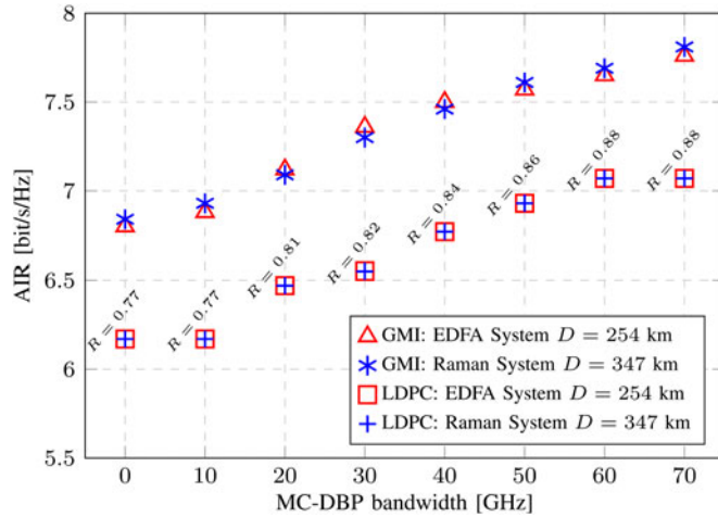
Fig. 5. AIR (at optimum launch power) as a function of MC-DBP BW using EDFA and Raman system.
