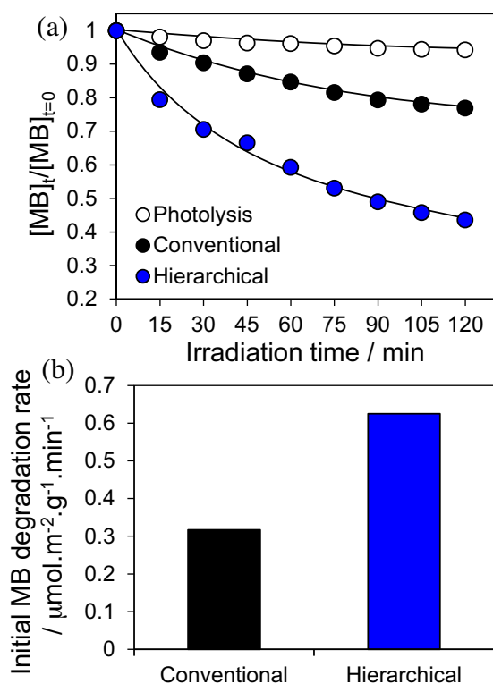
Fig. 7. (a) Visible light photocatalytic degradation of MB, and (b) normalised rates of MB degradation over conventional and hierarchical Cu 2 O nanocubes.
