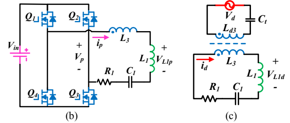
Fig. 5 (a) Schematic circuit with forward data transmission. (b) Power transfer equivalent circuit. (c) Data transmission equivalent circuit.
