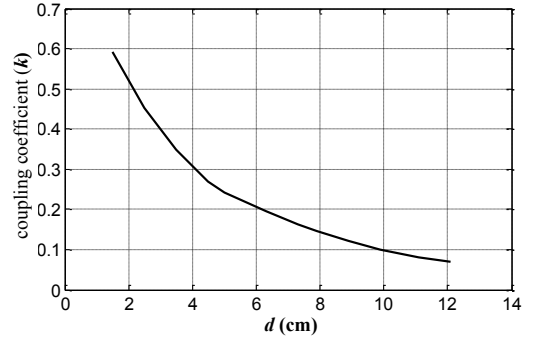
Fig. 13 Relationship between coupling coefficient and distance.
