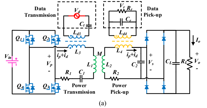
Fig. 4. SP compensation lumped circuit model.
