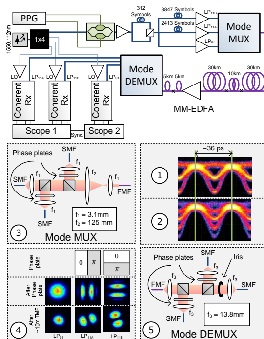
Fig. 1: Experimental Setup. (1) Optical 56-Gb/s QPSK eye, (2) Optical 112-Gb/s DP-QPSK eye, (3) 3-Modes (LP 01 , LP 11a and LP 11b ) multiplexer (Mode MUX) (4) Mode intensity profiles after phase plates and ~10m of two-mode fiber (TMF), (5) Mode de-multiplexer (Mode DEMUX)
