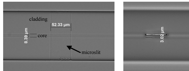
Fig. 2. Microscope images of the microslit fabricated into the fiber viewed along orthogonal planes.
