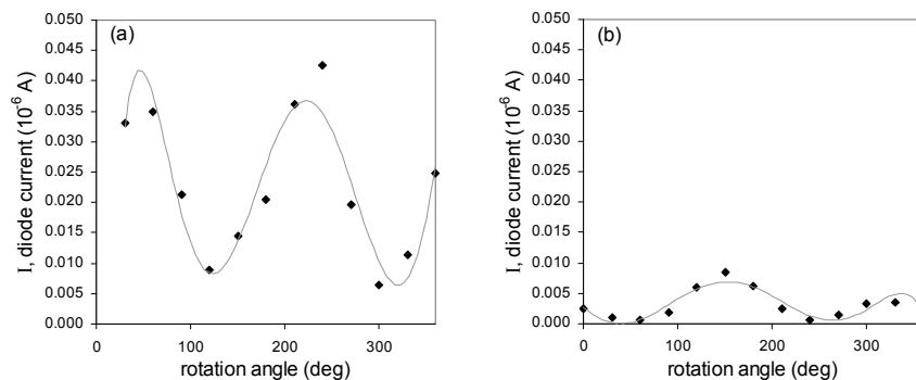
Fig. 3. Side-detection photodiode current versus rotation angle of the microslit when (a) n=1.333 and, (b) n=1.448 .
