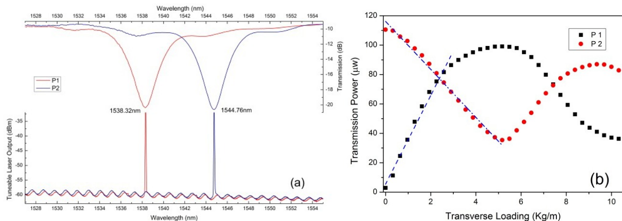
Figure 4(a) The upper plot is the transmission spectra of paired polarization peaks of 81°-TFG; the wavelength of the P1 loss peak is at
