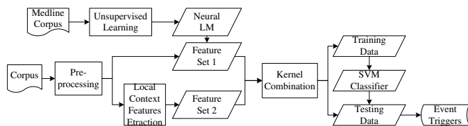
Fig. 1. The system architecture of our proposed framework for event trigger identification.
