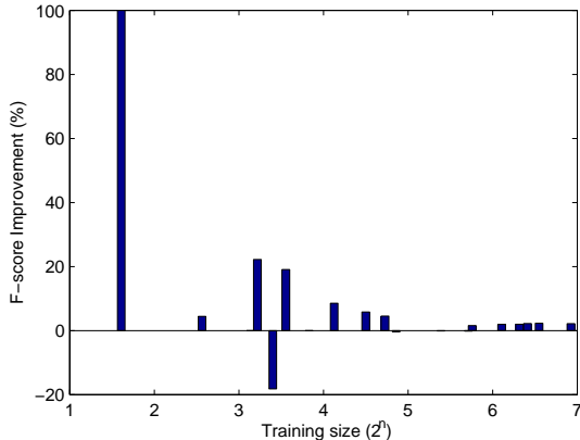
Fig. 2. Performance improvement vs size of training data in each event category.
