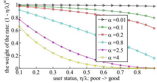
Fig. 3. The weight of the rate in utility function as a function of parameter \alpha .
