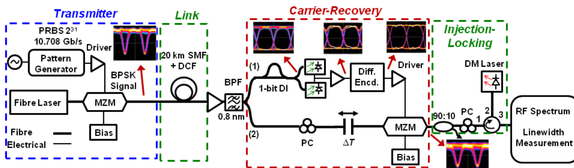
Fig. 1. Experimental arrangement for the dissemination scheme. List of acronyms: MZM: Mach-Zehnder Modulator, BPF: Band-pass filter, DI: Delayed interferometer, Diff. Encd. Differential Encoder, DM Laser: Discrete-Mode Laser, PC: Polarization controller, DCF: Dispersion compensating fibre, SMF: Single-mode fibre.
