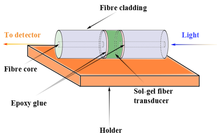
Figure 8. Example of an AFCOS sensor, adapted from [124].
