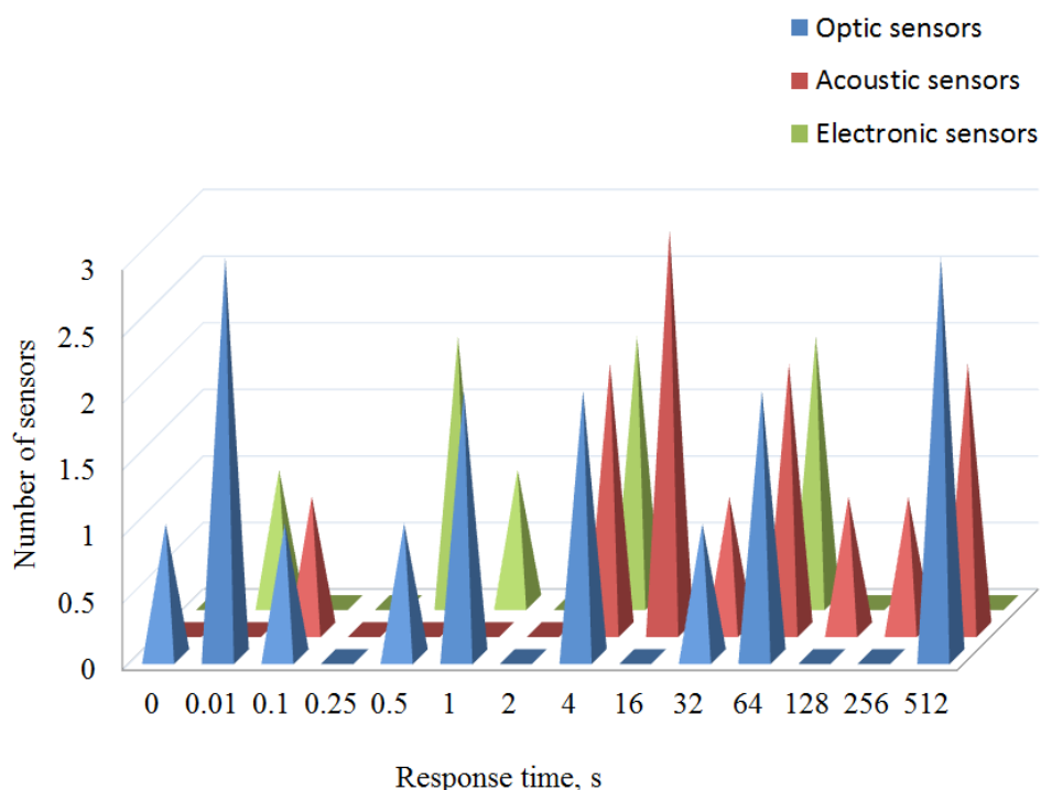
Figure 2. Response times of different types of humidity sensors.
