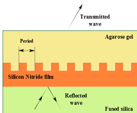
Figure 9. The guided-mode resonance sensor configuration, adapted from [125].
