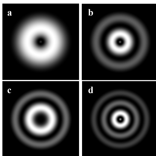
Figure 6. The intensity distribution of the first cladding modes (a) l = 1, \nu = 1 ; (b) l = 1, \nu = 3 ; (c) l = 1, \nu = 4 ; (d) l = 1, \nu = 5 . The modes were simulated using [105].
