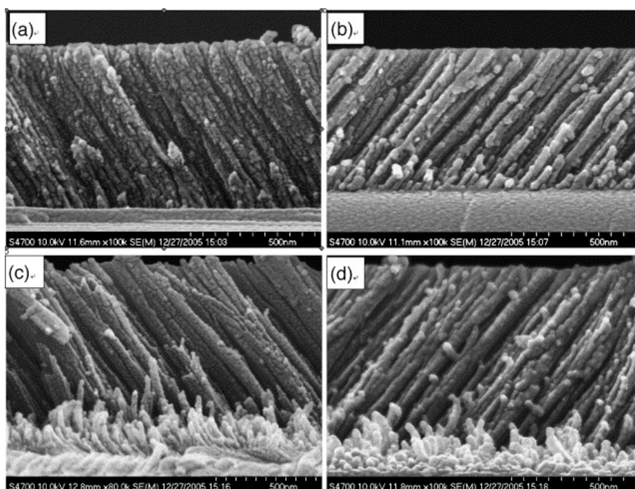
Figure 3. Cross-sectional SEM images of the thin TiO 2 films deposited at different flux angles. (a) \alpha = 60^\circ ; (b) \alpha = 70^\circ ; (c) \alpha = 75^\circ ; (d) \alpha = 80^\circ , reproduced from [31] with permission.
