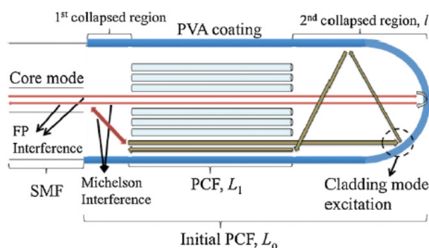
Figure 5. The sensor based on PVA coated photonic crystal interferometer, reproduced from [94] with permission.
