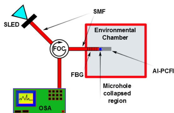
Figure 7. Schematic diagram of the hybrid fiber optic sensor system for simultaneous measurement of RH and temperature. (SLED—Super luminescent diode. FOC—Fiber optic circulator. SMF—Single mode fiber. FBG—Fiber Bragg grating. AI-PCFI—Agarose infiltrated-photonic crystal fiber interferometer. OSA—Optical spectrum analyzer. Dotted arrows represent the light path), adapted from [114].
