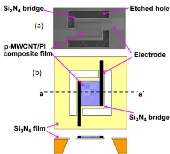
Figure 4. (a) Scanning electron microscope (SEM) image of active layer; and (b) schematic view of the resistive-type RH sensors based on p -MWCNT-PI composite film, reproduced from [17] with permission.
