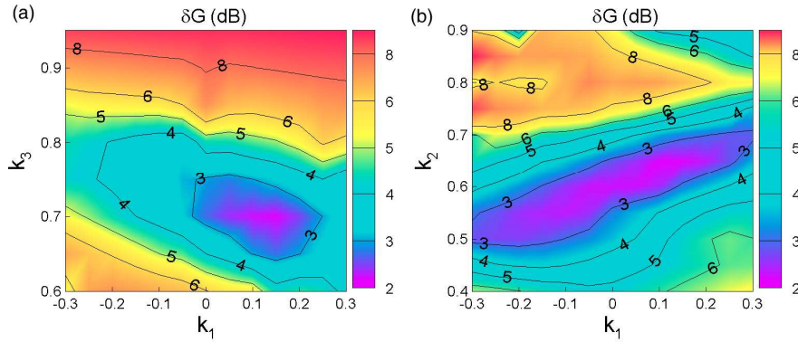
Fig. 2. (a) Contour plot of \delta G in the plane of optimization parameters ( k_1, k_3 ) for a fixed k_2 = 0.64 ; (b) Contour plot of \delta G in the plane of optimization parameters ( k_1, k_2 ) for a fixed k_3 = 0.7 .
