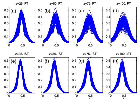
Fig. 4. Eye diagram for the signals reconstructed via FT, (a) at z = 25 , (b) at z = 50 , (c) at z = 75 , and (d) at z = 100 ; and via IST, (e) at z = 25 , (f) at z = 50 , (g) at z = 75 , and (h) at z = 100 .
