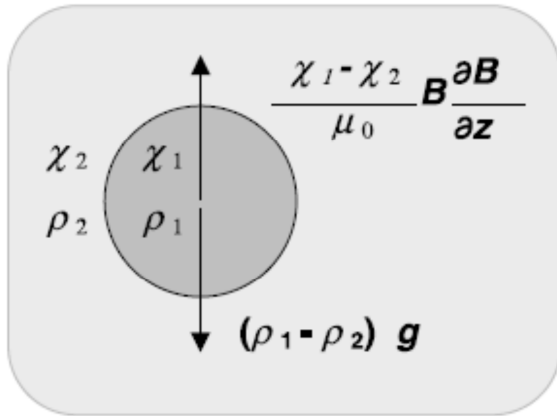
a. Forces balance(in the centre )
