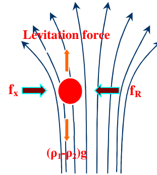
b. Forces balance(deviate from the centre)
