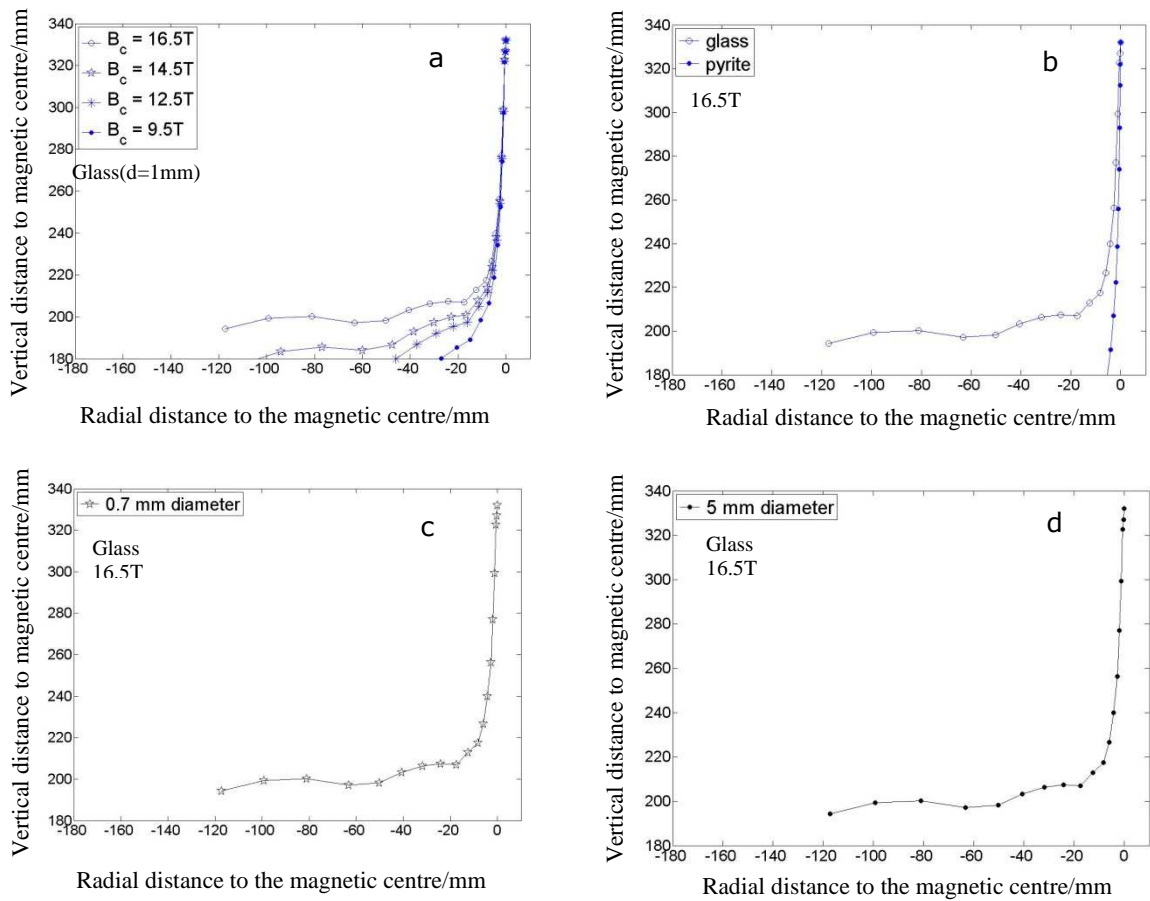
Fig. 7 Simulation results of particle deflection in magnetic field
