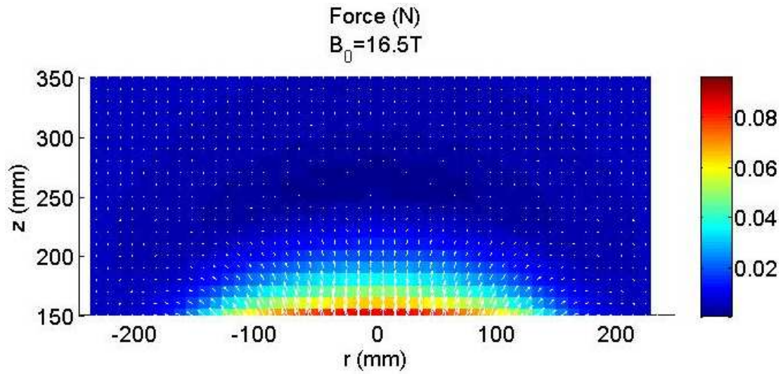
Fig. 6 Forces acted on glass particle ( d=1\text{mm} ) in magnetic field ( B_c=16.5\text{ T} )
