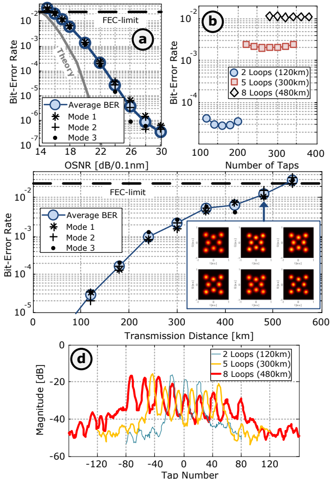
Fig. 2.a) Back-to-back curve, b) Tap sweep for 120, 300 and 480 km, c) Distance sweep, d) Impulse response after 120, 300 and 480 km
