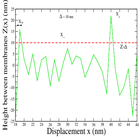
Fig. 1: A 1D profile of a 2D membrane fluctuating around the line \langle Z \rangle = 0 , from simulated data. X_+ & X_- are the respective sizes of the patches above and below the threshold depth Z = \Delta = 10 nm.
