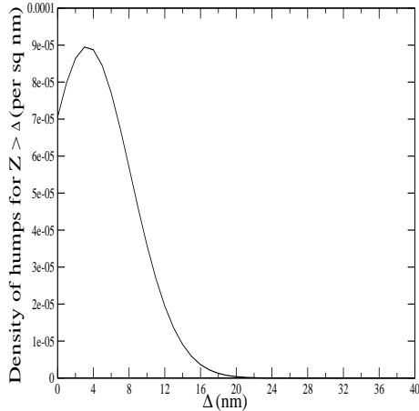
Fig. 3: Probability density of humps around the line Z = \Delta as a function of the average threshold \Delta (nm) as predicted from Eq. (9)
