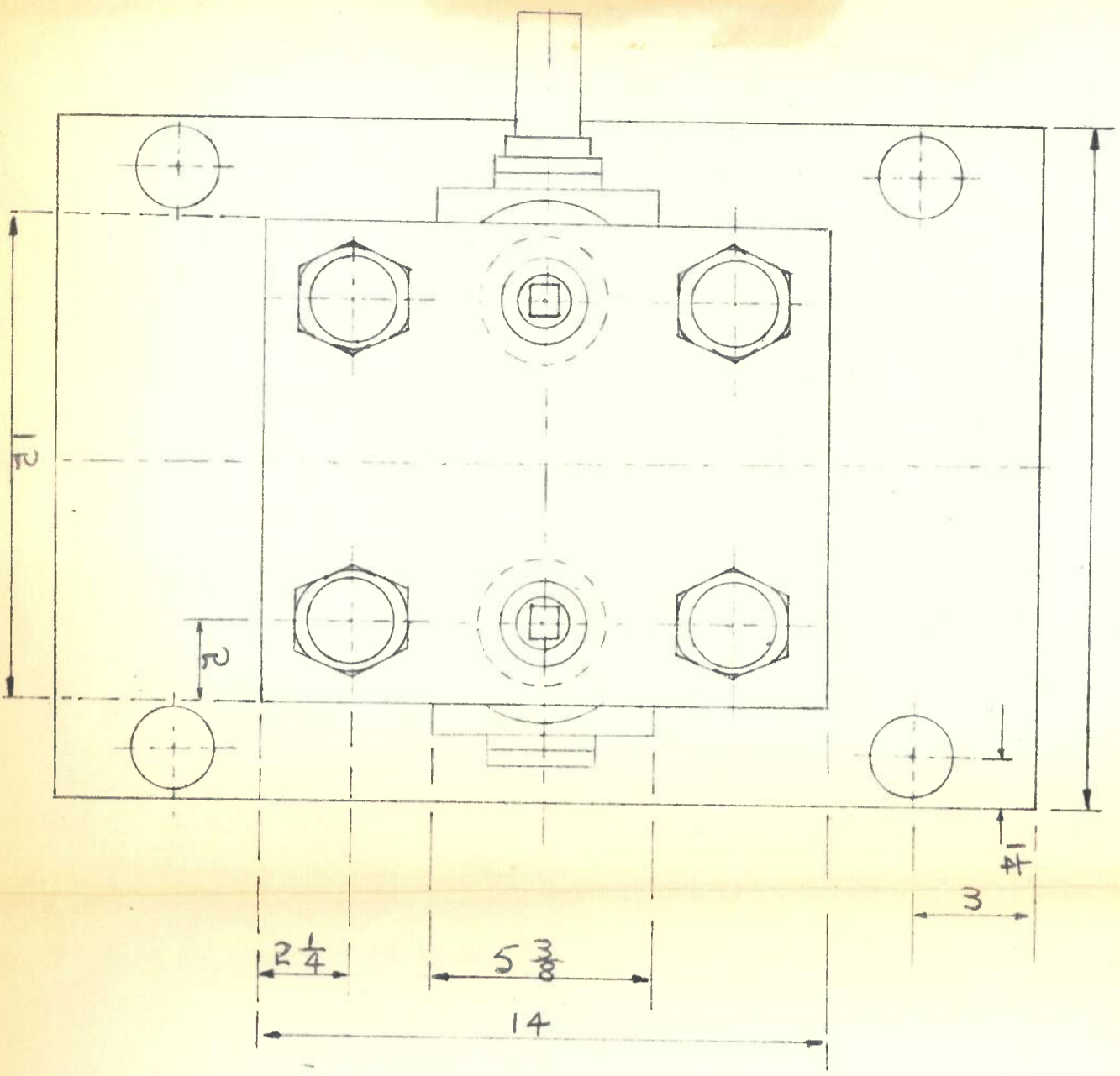
Figure A1. DESIGN OF THE MILL HOUSING.
