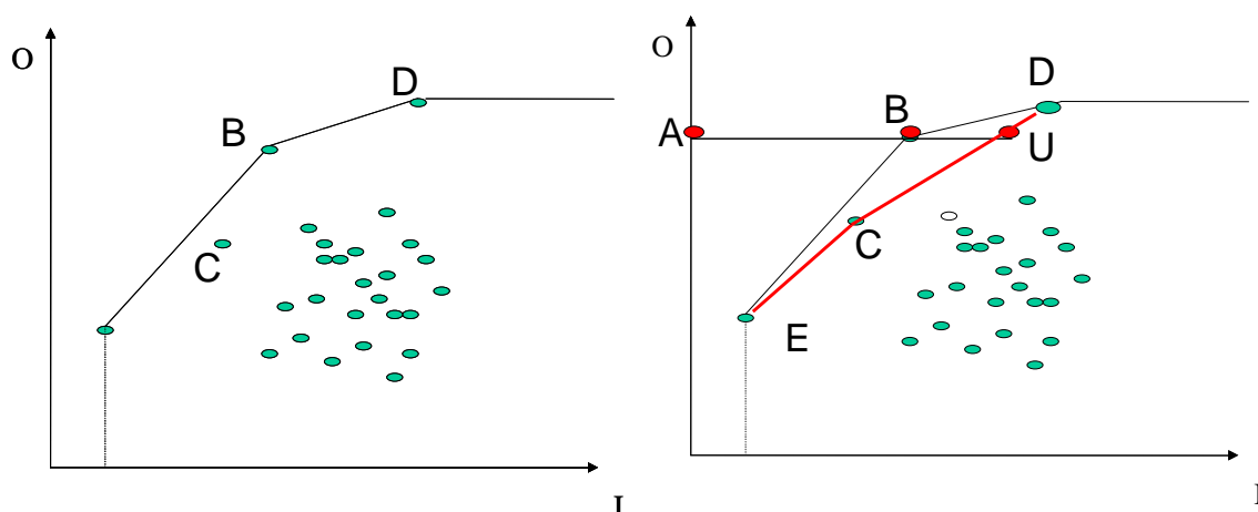
Figure 1: The identification of outliers
