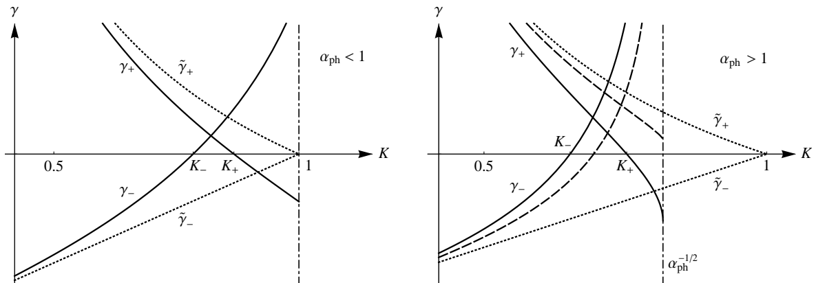
Figure 1: Weak tunneling ( \gamma_+ ) and weak scattering ( \gamma_- ) exponents as functions of the Luttinger parameter K < 1 for a weak (a) or strong (b) el-ph coupling ( \alpha_{\text{ph}} = 0.7 and \alpha_{\text{ph}} = 1.5 were used). The dotted lines represent \tilde{\gamma}_{\pm} for the phononless LL, the solid and dashed lines correspond to \beta_{\text{F}} < \beta_{\text{F}}^* and \beta_{\text{F}} > \beta_{\text{F}}^* , respectively (we used \beta_{\text{F}} = 0.5 and \beta_{\text{F}} = 1.5 respectively). The latter is shown only for the strong coupling where for \beta_{\text{F}} > \beta_{\text{F}}^* the exponent \gamma_+ does not change sign within the stability region, K < \alpha_{\text{ph}}^{-1/2} .
