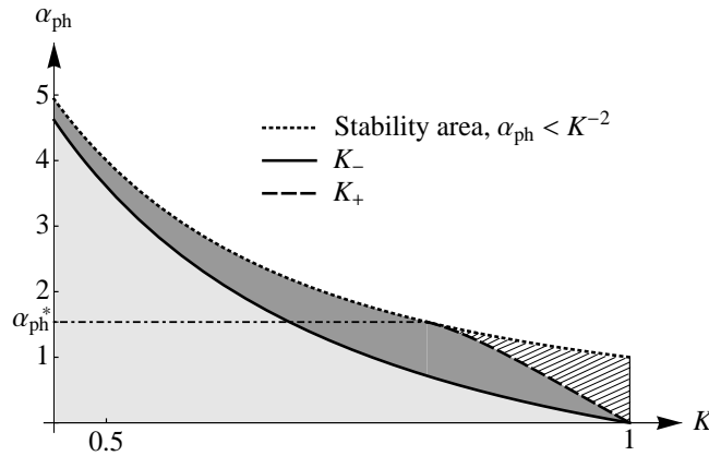
Figure 2: Phase diagram: The light-grey area represents the insulating regime. In the dark-grey area there exists a line of unstable fixed points separating the metallic state for a weak scatterer from the insulating phase for a strong one. The hatched area (reachable only for \alpha_{\text{ph}} < \alpha_{\text{ph}}^* ) corresponds to the purely metallic phase. We used \beta_{\text{F}} = 1.1 .
