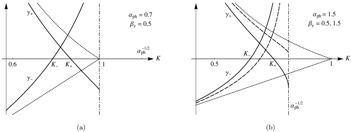
FIG. 1. Weak tunneling ( \gamma_+ ) and weak scattering ( \gamma_- ) exponents as functions of the Luttinger parameter K < 1 for a weak (a) or strong (b) el-ph coupling, ( \alpha_{\text{ph}} \leq 1 , respectively). The dotted lines represent \tilde{\gamma}_{\pm} for the phononless LL, the solid and dashed lines correspond to \beta_{\text{F}} \equiv v_{\text{F}}/c = 0.5 and \beta_{\text{F}} = 1.5 , respectively. The latter is shown only for the strong coupling where for \beta_{\text{F}} > [\alpha_{\text{ph}}(\alpha_{\text{ph}} - 1)]^{-1/2} the exponent \gamma_+ does not change sign within the stability region, K < \alpha_{\text{ph}}^{-1/2} .
