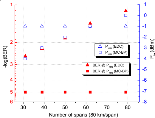
Fig. 3 Minimum achievable BER (left axis, red) and required P_{\min} per channel per span, observed for the given system (right axis, blue) versus number of fibre spans by using EDC alone (triangles) and full-bandwidth back-propagation (squares) for a system without inline optical dispersion compensation (PM-4QAM).
