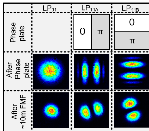
Fig. 2. Mode intensity profiles after phase plates (middle row) and after \sim 10 m of FMF (bottom row).
