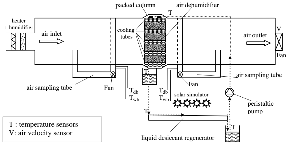
Fig. 1. Schematic diagram of the experimental rig.
