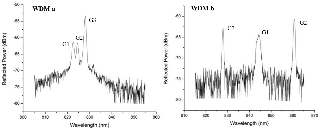
Figure 6 a: WDM sensor using a single phase mask and utilising thermal annealing, b: WDM sensor using two separate phase masks and a single thermal annealing stage.
