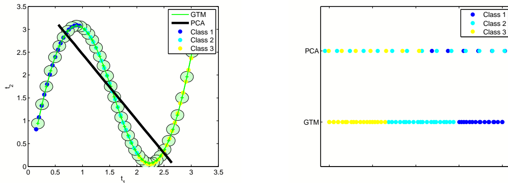
(a) The function t_2 = t_1 + 2.25 \sin(2t_1) is divided into three classes, depending on the value of t_1 .
