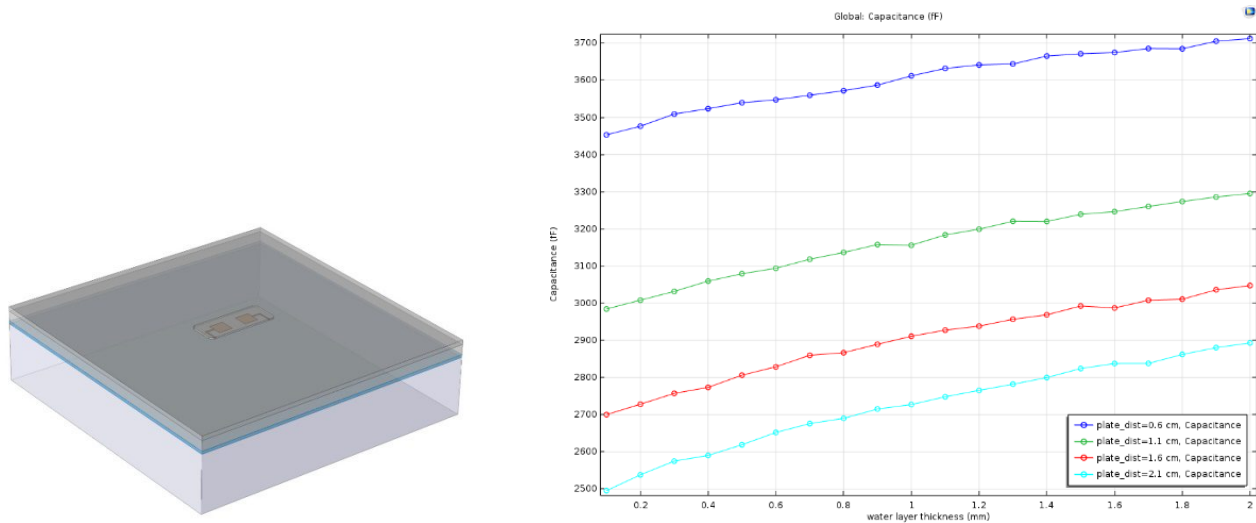
Figure 4b. Geometric setup for the second simulation. A capacitor is placed on top of a human head with layers of skin, skull bone, and cerebrospinal fluid ( left ). The change in volume of the CSF is plotted against the change in capacitance for different configurations of the capacitor ( right ).
