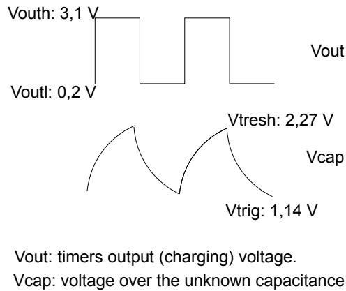
Figure 2. Signals and voltages of the capacitance measuring device.
