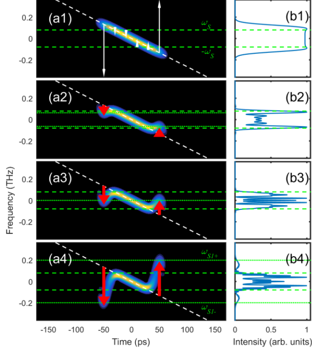
Figure 6: Spectro-temporal representation of a fourth-order super-Gaussian pulse at different propagation distances in the fibre: z = 0 , z = 62 m, z = z_{SJ} , and z = 300 m (panels 1 to 4, respectively). Subplots (a) and (b) show the spectrograms and the spectral intensity profiles, respectively. The white dashed lines represent the slope coefficient of the pulse chirp at the fibre input. The green dashed and dotted lines represent the theoretical predictions for \pm\omega_S and \omega_{SJ\pm} , respectively. The white arrows have a length proportional to the temporal gradient of the pulse intensity profile. The red arrows represent the frequency shift at t = T_{fwhm}/2 .
