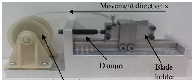
Fig. 3: New passive and portable POF cleaver
