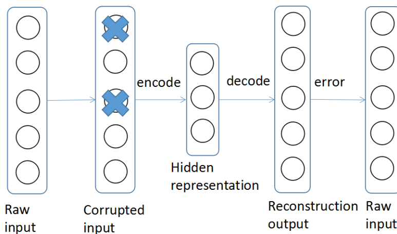
Fig. 3. A graphic structure of SDAE.
