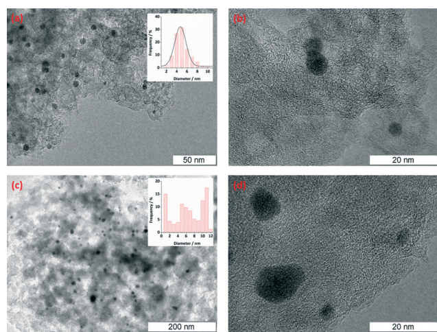
Fig. 2 HR-TEM microscopic images of Pd nanoparticles on (a–b) Pd/triC fresh catalysts; (c–d) Pd/biC fresh catalysts.
